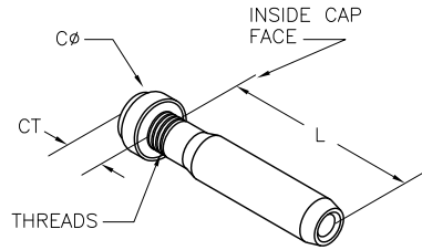
FIXED CAP END, STAINLESS STEEL
